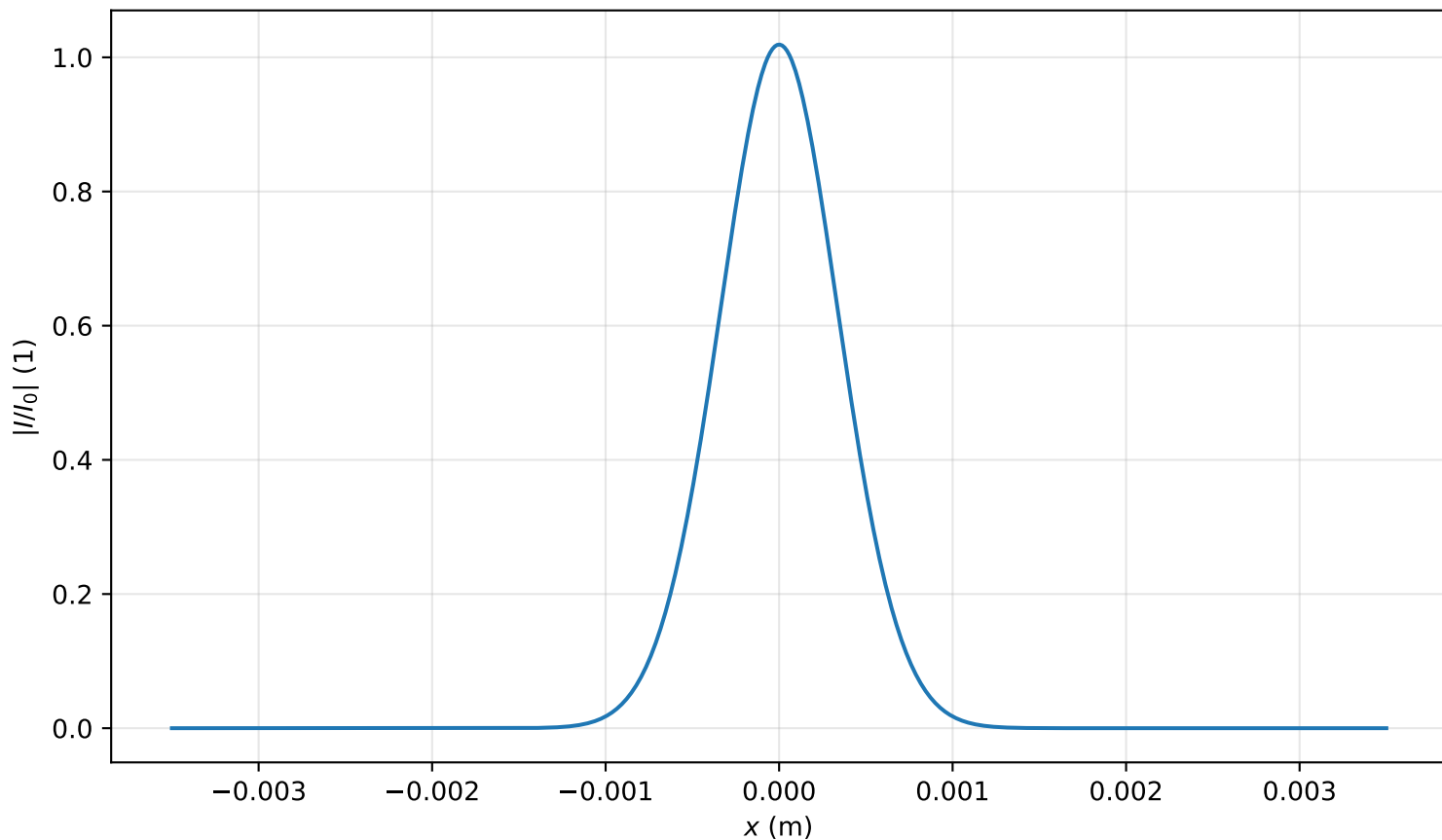
Intensity profile I(x, y = 0, z = 0.239m)/I_0 , P_{in}=0.6P_{cr} , artificial time
